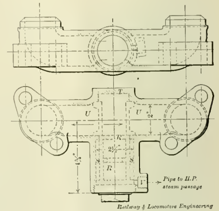
BY-PASS OF ROGERS COMPOUND.
